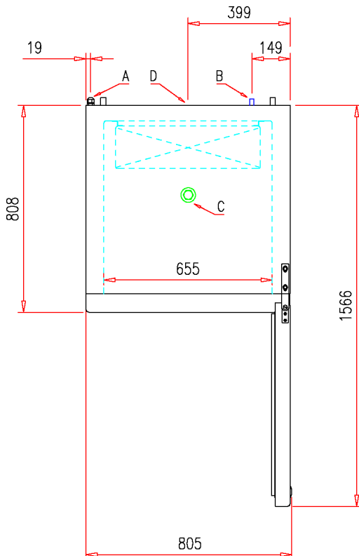
Top View
