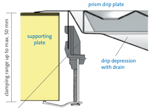
cross section supporting plate / drip tray (top side assembly)
