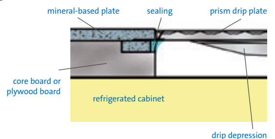
cross section supporting plate / drip tray (bottom side assembly)
