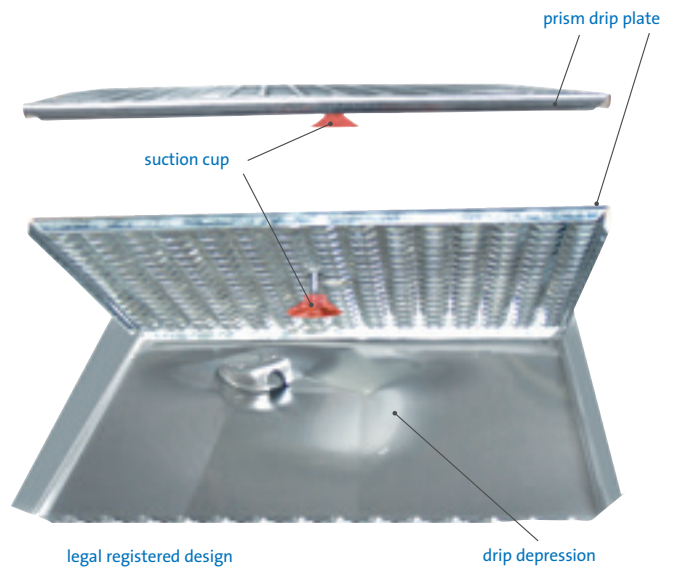
Suction cup for fixing the prism drip plates is used for mobile sectors.
